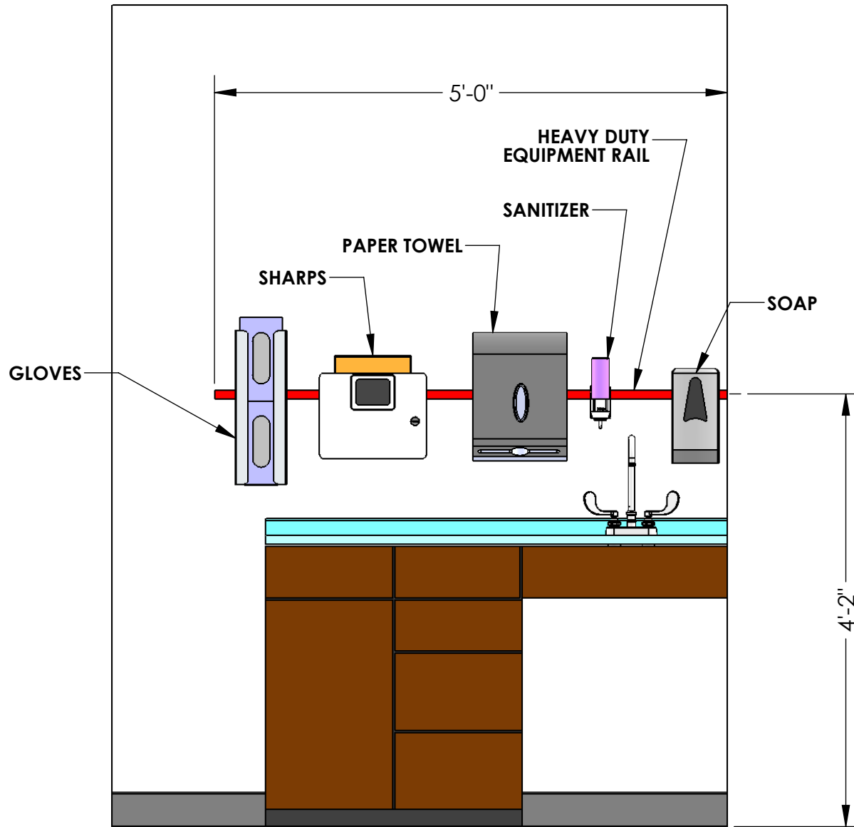
EQUIPMENT RAIL ELEVATION INFECTION CONTROL #2
