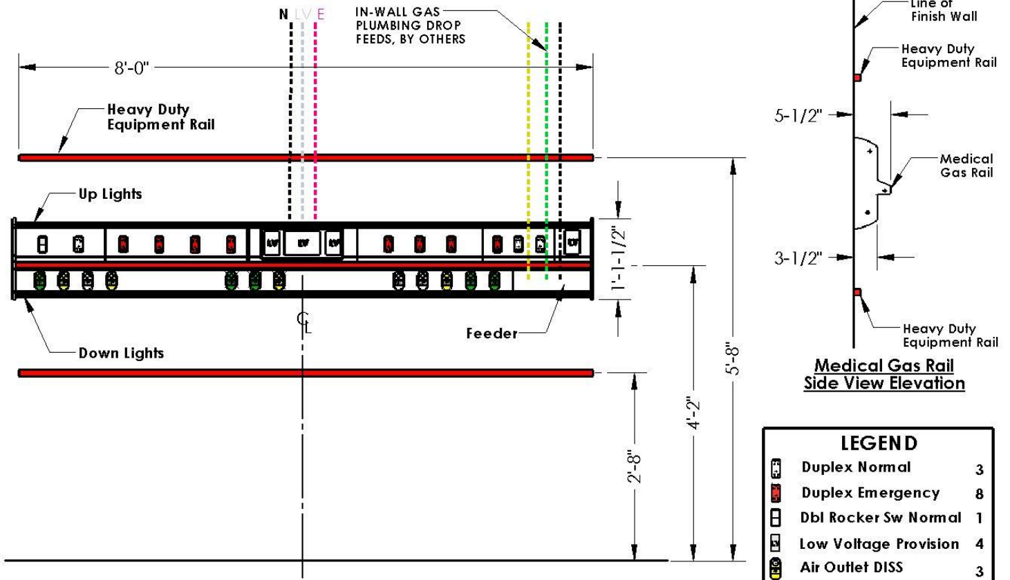
TYPICAL MEDICAL GAS RAIL HEADWALL
