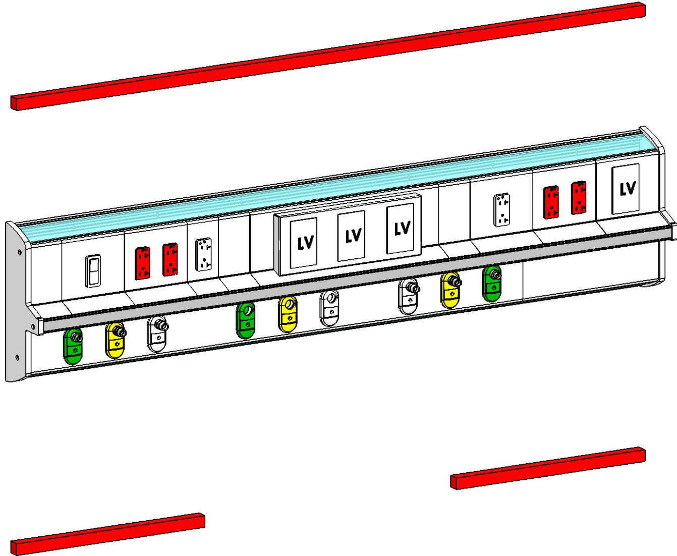
STANDARD 5 FOOT MEDICAL GAS RAIL HEADWALL ISOMETRIC VIEW
